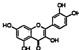
QUERCETIN
